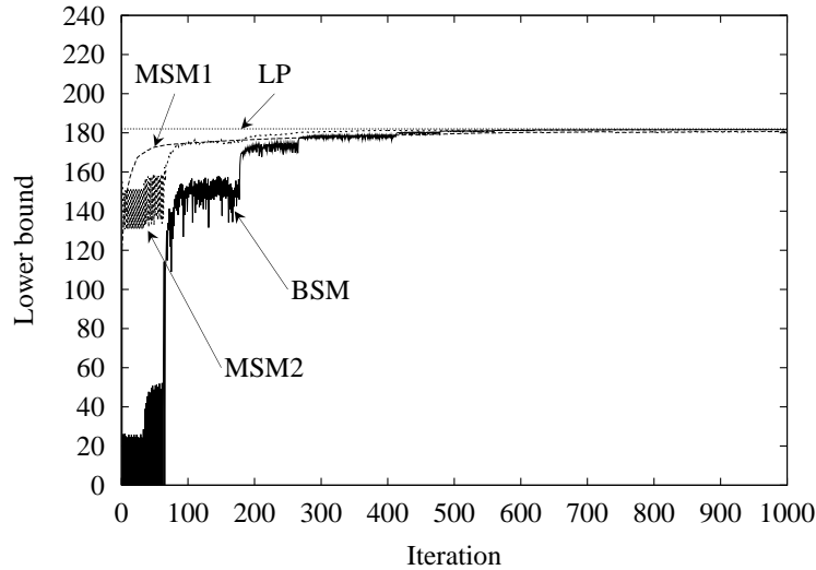
Figure 1: Comparison of the subgradient methods BSM, MSM1 and MSM2 on instance RAIL516
