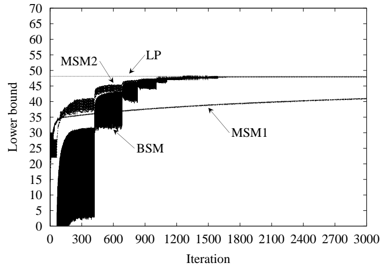
Figure 2: Comparison of the subgradient methods BSM, MSM1 and MSM2 on instance H.1
