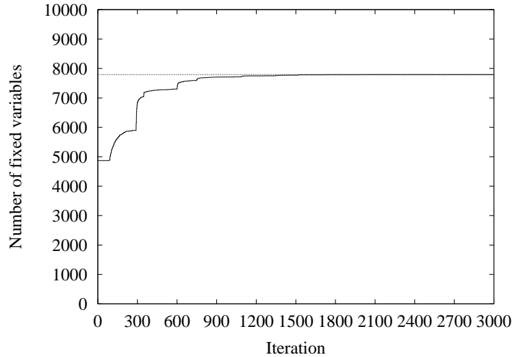
Figure 3: Number of fixed variables at every iteration on instance H.1
